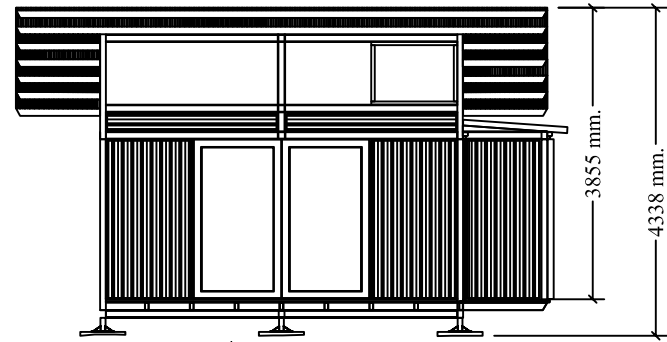
NORTH ELEVATION
