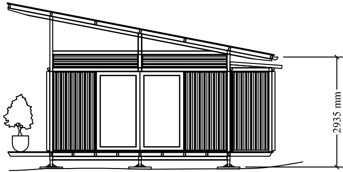
EAST ELEVATION
